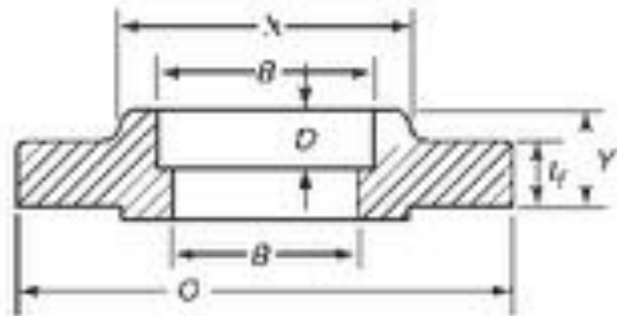
Socket Welding
