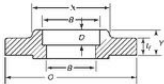
Socket Welding
